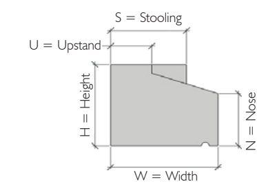
Section of stooped cill
